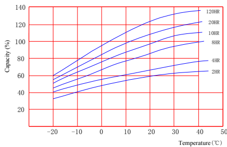
Figure 3 Relation curves between capacity and temperature
