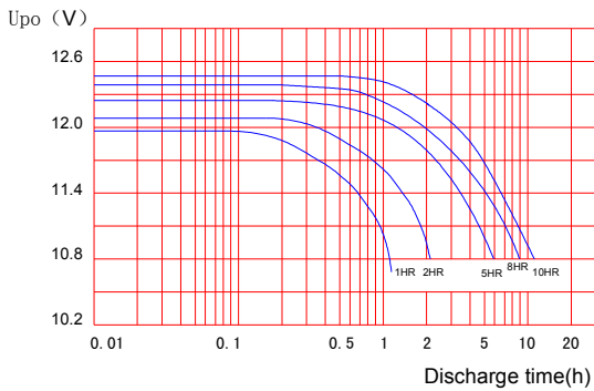
Figure 1 Discharge characteristic curve (20°C)
