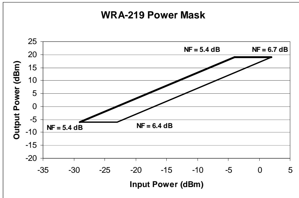
Figure 1: Power mask with noise figures 1 for WRA-219
